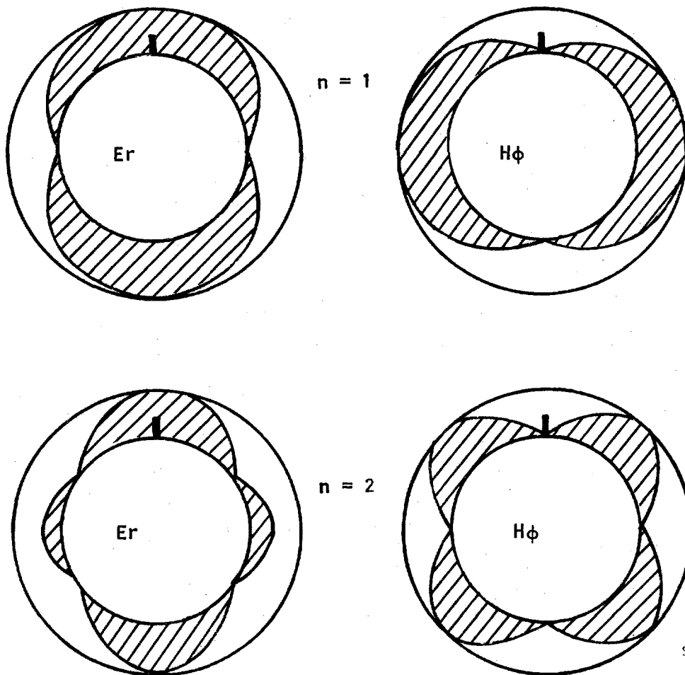
Figure 7-2. Standing Waves of the Radial Electric and Horizontal Magnetic Field in a Concentric Shell Cavity Excited by a Vertical Electric Radiator at the Two Lowest Frequencies (after Reference 7-2, p. 41). (These Waves are also Called Schumann Waves.)
